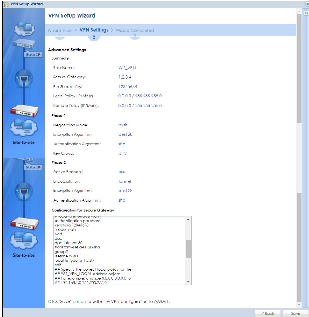
Figure 150 VPN Advanced Wizard: Summary
