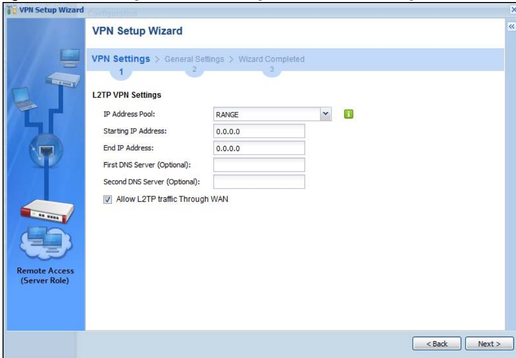
Figure 107 VPN Settings for L2TP VPN Settings Wizard: L2TP VPN Settings
