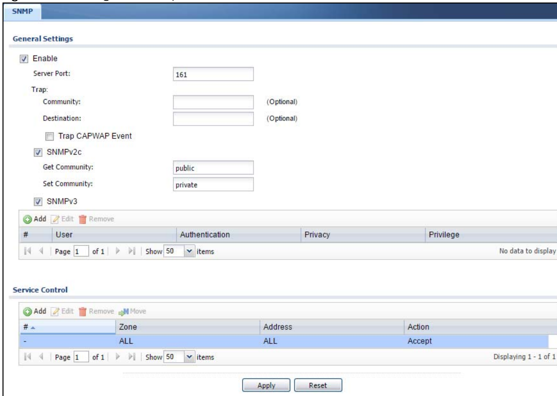
Figure 688 Configuration > System > SNMP
