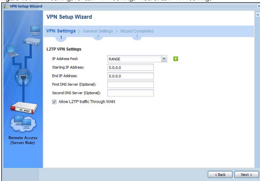
Figure 164 VPN Settings for L2TP VPN Settings Wizard: L2TP VPN Settings
