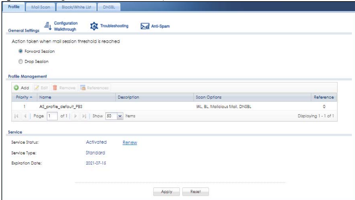
Figure 526 Configuration > UTM Profile > Anti-Spam > Profile
