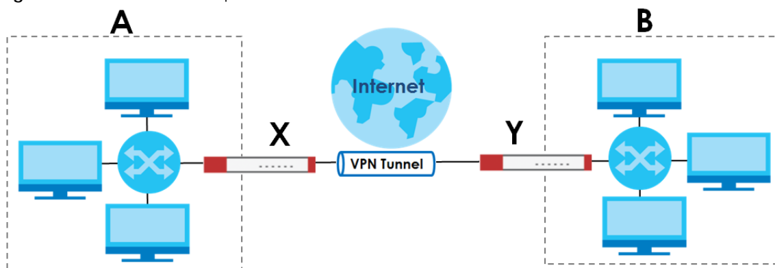
Figure 438 IPSec VPN Example
